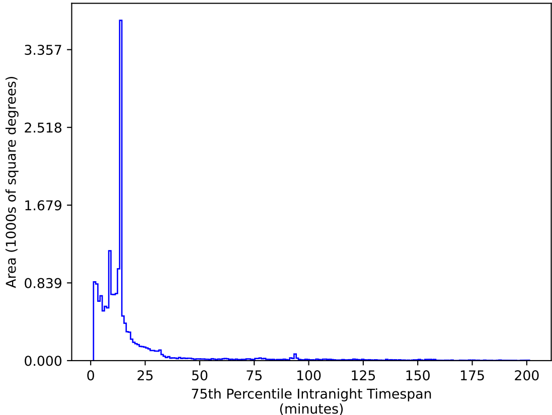
reweight_plane_v3.3_10yrs WFD z band: 75th Percentile Intranight Timespan
