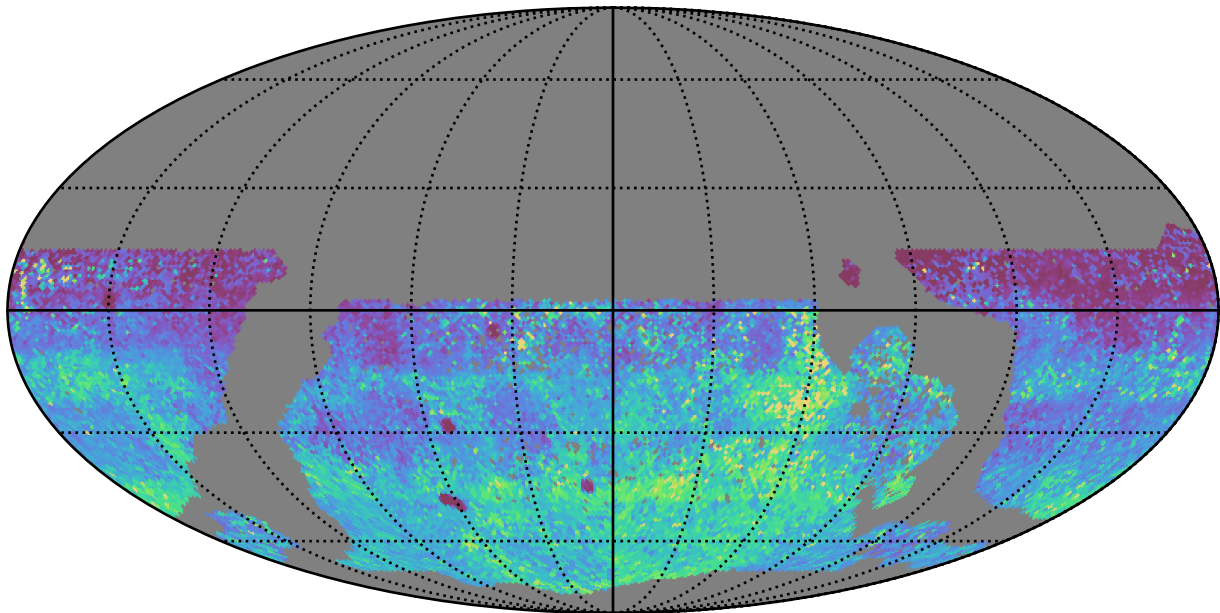
reweight_plane_v3.3_10yrs WFD y band: 75th Percentile Intranight Timespan
