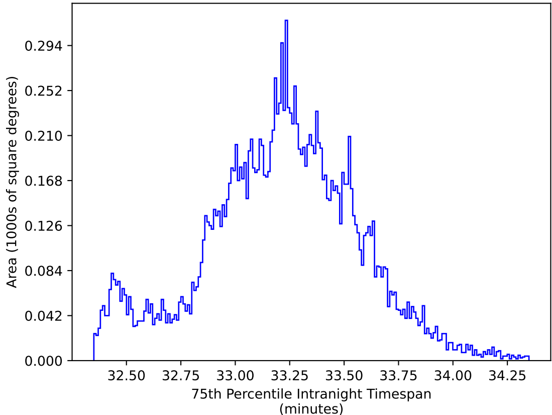
reweight_plane_v3.3_10yrs WFD y band: 75th Percentile Intranight Timespan
