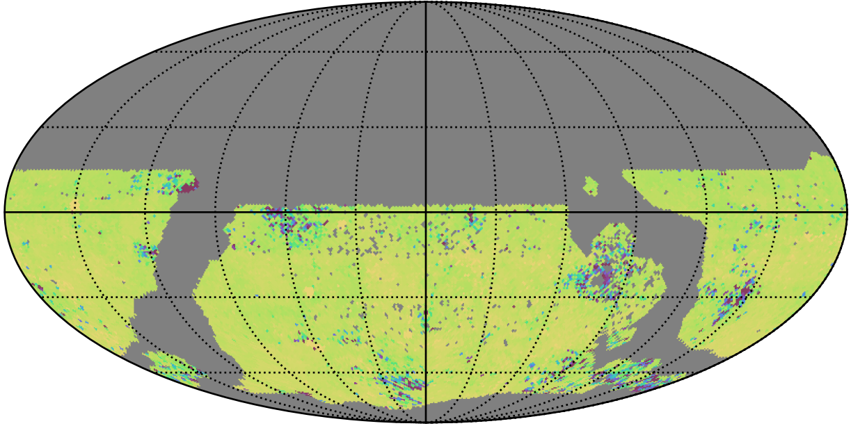
reweight_plane_v3.3_10yrs WFD ug bands: 75th Percentile Intranight Timespan
