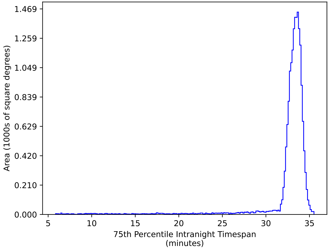
reweight_plane_v3.3_10yrs WFD ug bands: 75th Percentile Intranight Timespan
