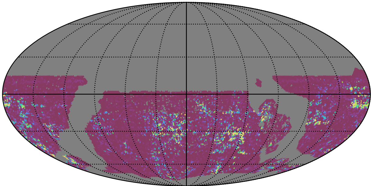
reweight_plane_v3.3_10yrs WFD u band: 75th Percentile Intranight Timespan
