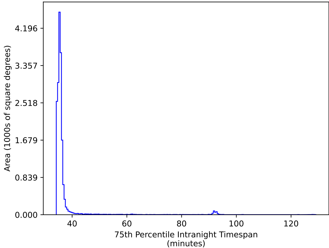
reweight_plane_v3.3_10yrs WFD ri bands: 75th Percentile Intranight Timespan
