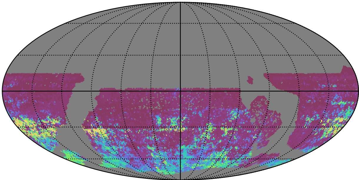
reweight_plane_v3.3_10yrs WFD r band: 75th Percentile Intranight Timespan
