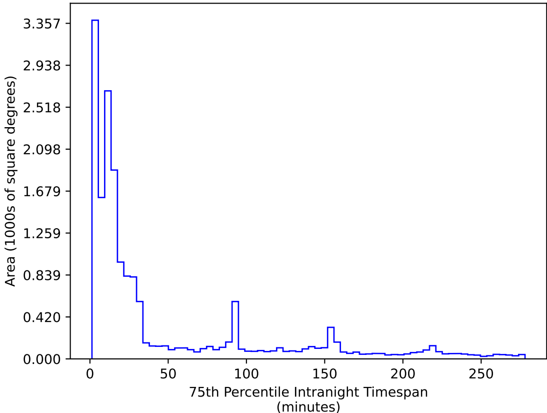
reweight_plane_v3.3_10yrs WFD r band: 75th Percentile Intranight Timespan
