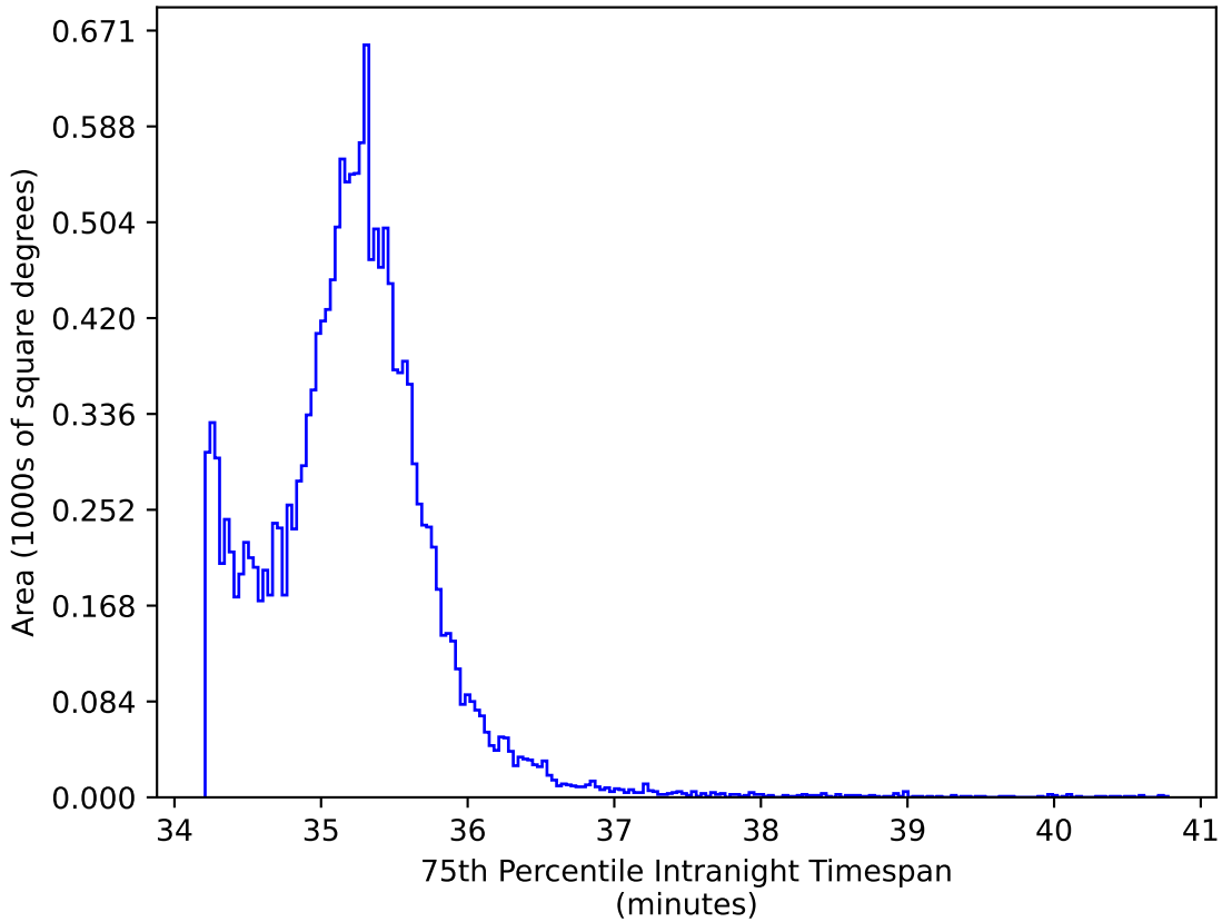
reweight_plane_v3.3_10yrs WFD iz bands: 75th Percentile Intranight Timespan
