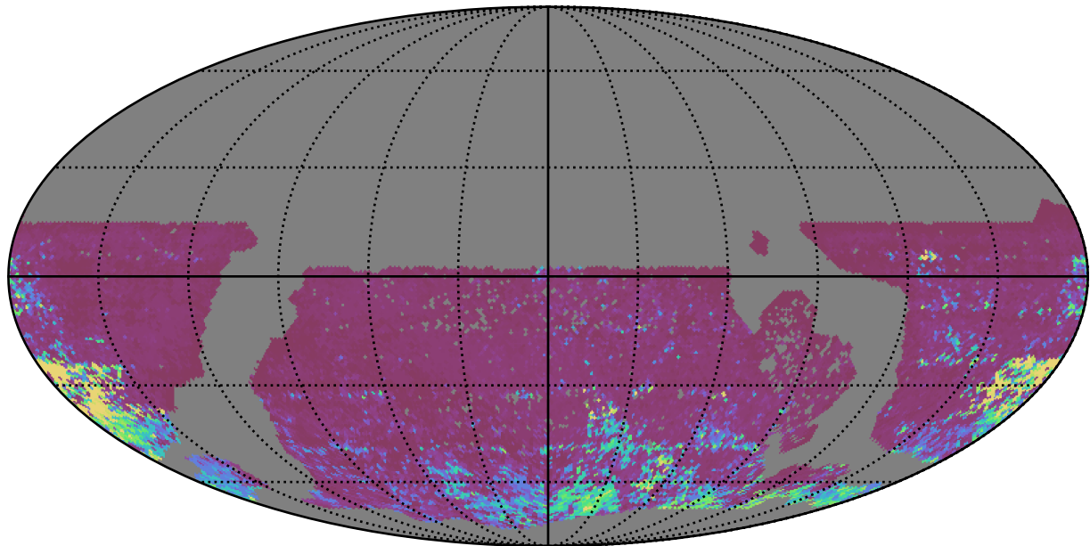
reweight_plane_v3.3_10yrs WFD i band: 75th Percentile Intranight Timespan
