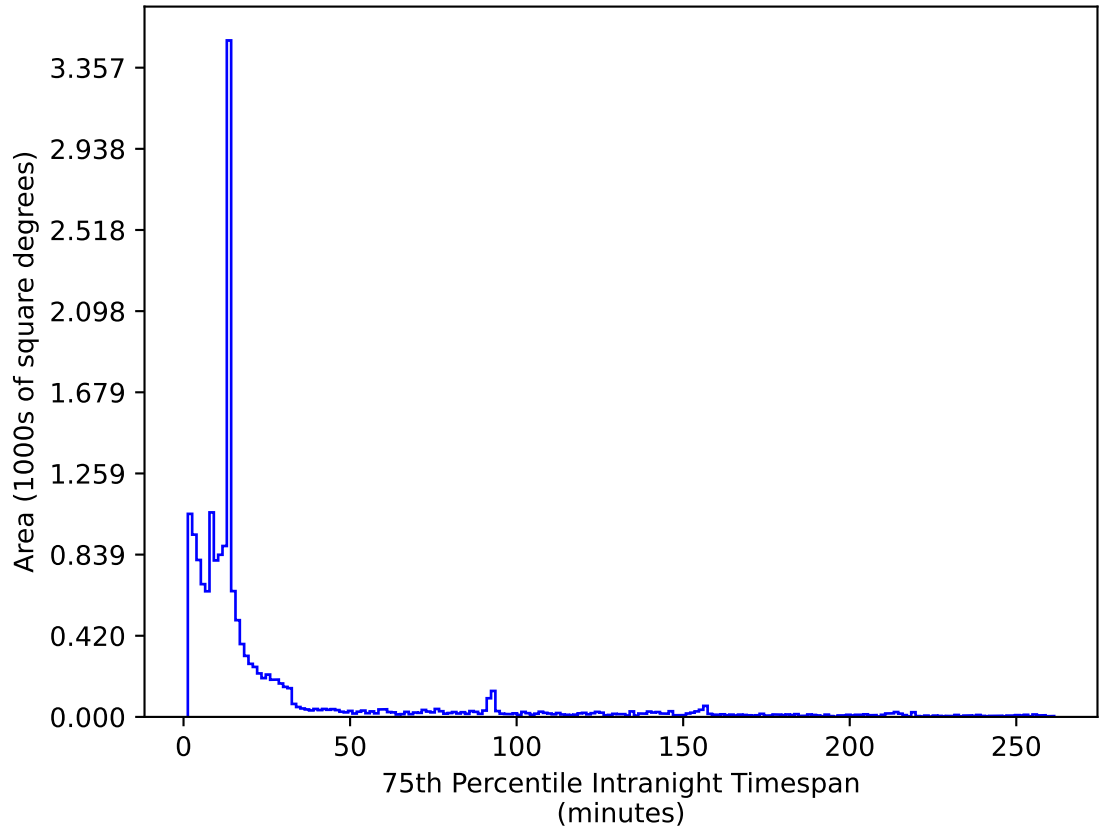
reweight_plane_v3.3_10yrs WFD i band: 75th Percentile Intranight Timespan
