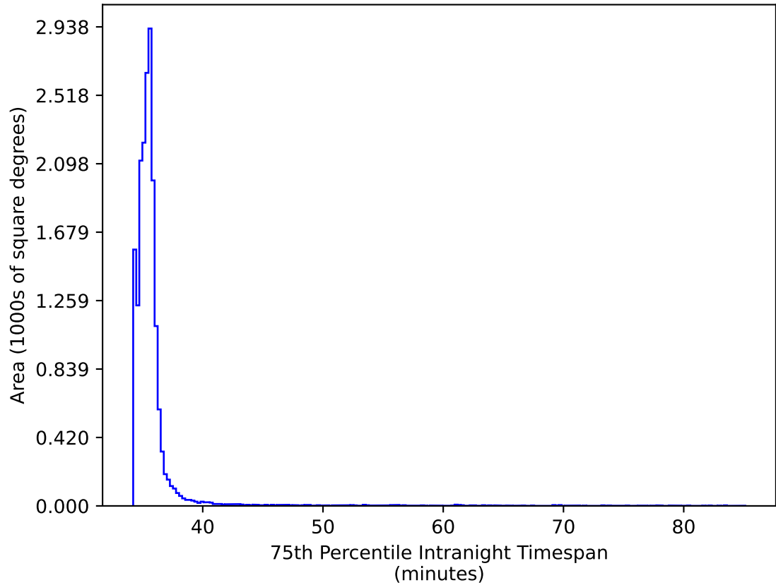
reweight_plane_v3.3_10yrs WFD gr bands: 75th Percentile Intranight Timespan
