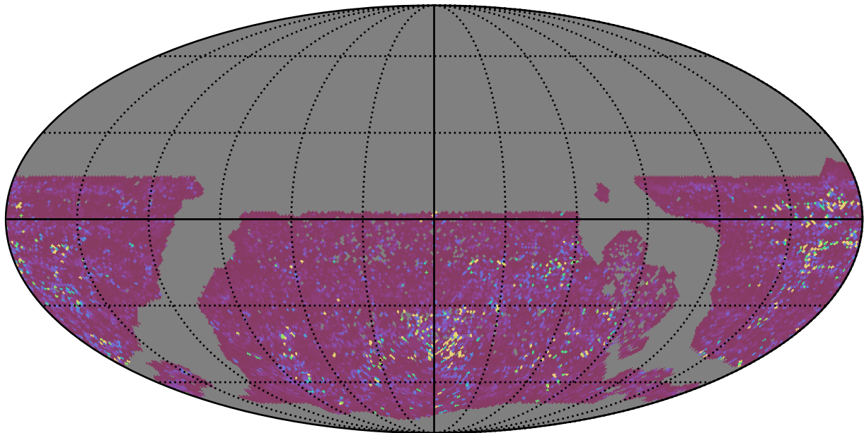
reweight_plane_v3.3_10yrs WFD g band: 75th Percentile Intranight Timespan
