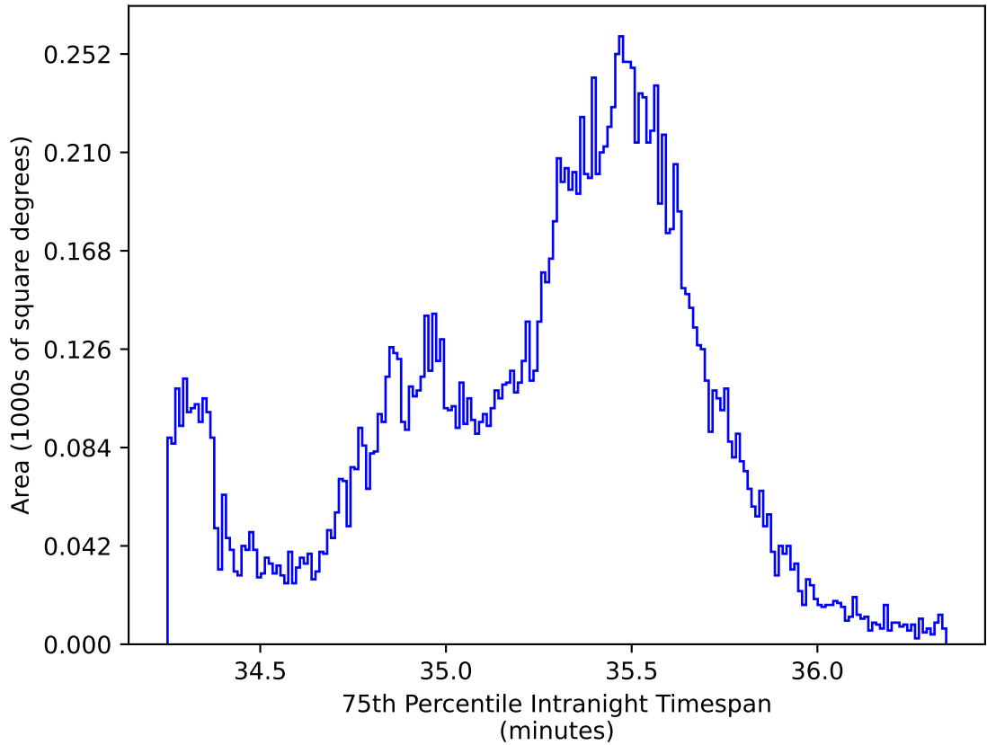
reweight_plane_v3.3_10yrs WFD all bands: 75th Percentile Intranight Timespan
