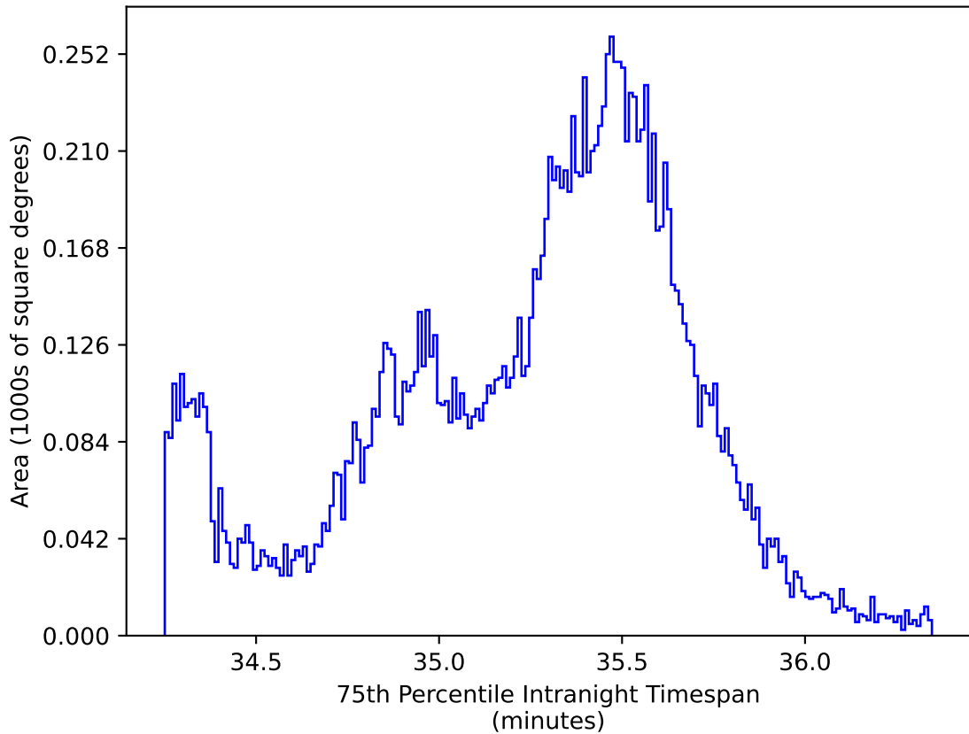
reweight_plane_v3.3_10yrs WFD: 75th Percentile Intranight Timespan
