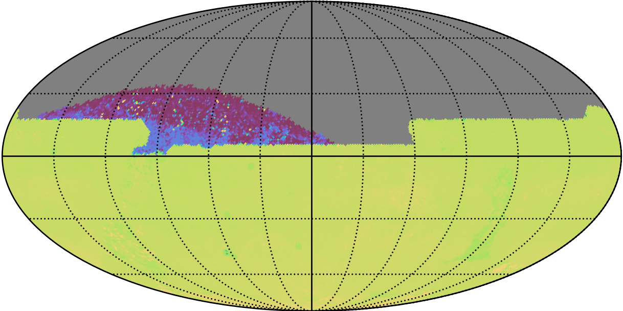
reweight_plane_v3.3_10yrs All sky zy bands: 75th Percentile Intranight Timespan
