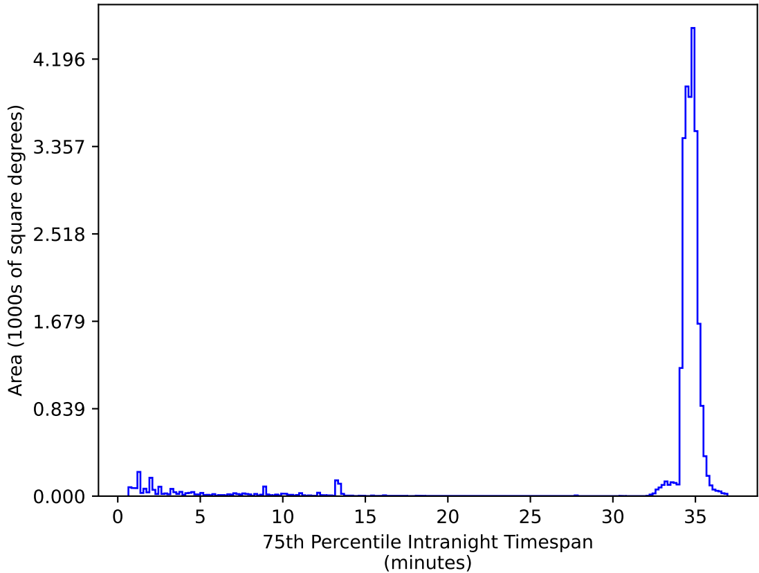
reweight_plane_v3.3_10yrs All sky zy bands: 75th Percentile Intranight Timespan
