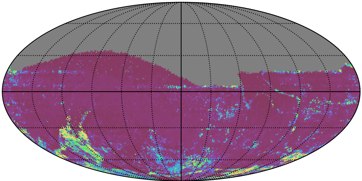
reweight_plane_v3.3_10yrs All sky z band: 75th Percentile Intranight Timespan
