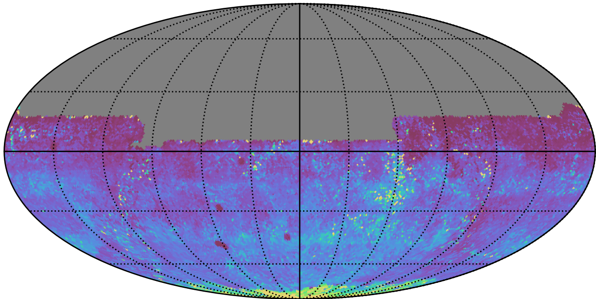
reweight_plane_v3.3_10yrs All sky y band: 75th Percentile Intranight Timespan
