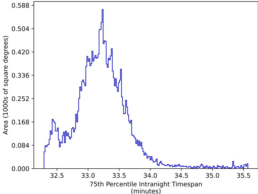
reweight_plane_v3.3_10yrs All sky y band: 75th Percentile Intranight Timespan
