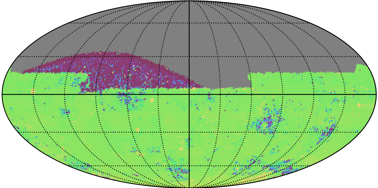
reweight_plane_v3.3_10yrs All sky ug bands: 75th Percentile Intranight Timespan
