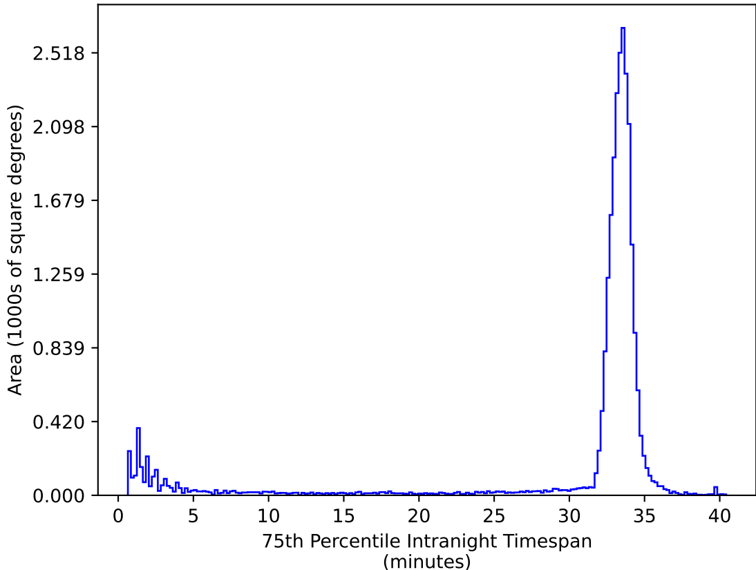
reweight_plane_v3.3_10yrs All sky ug bands: 75th Percentile Intranight Timespan
