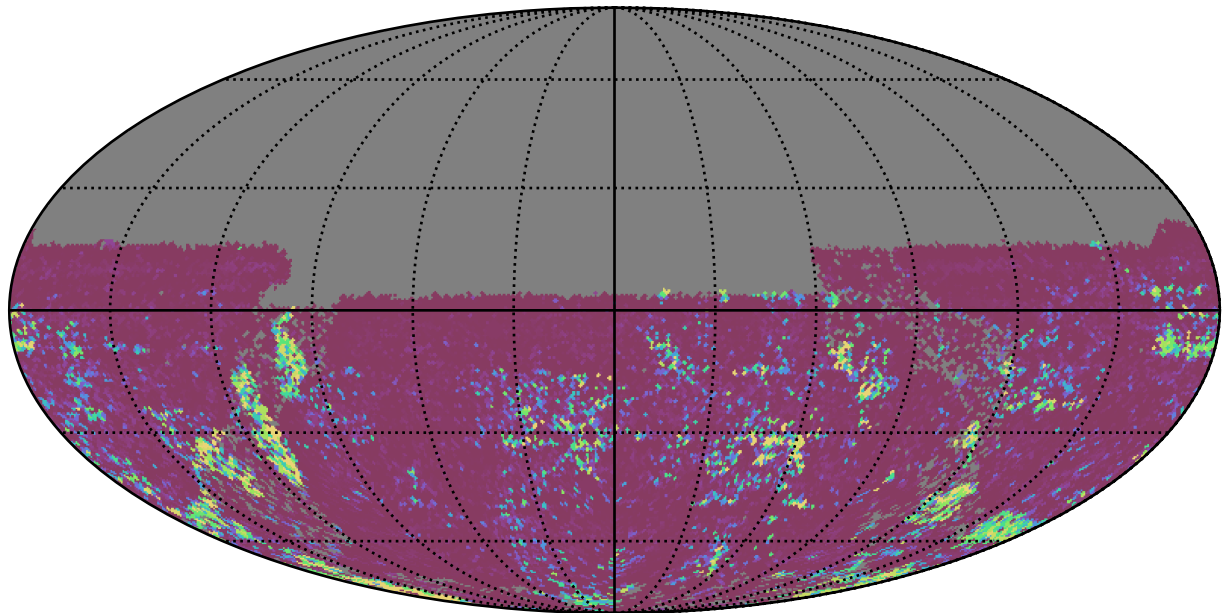
reweight_plane_v3.3_10yrs All sky u band: 75th Percentile Intranight Timespan
