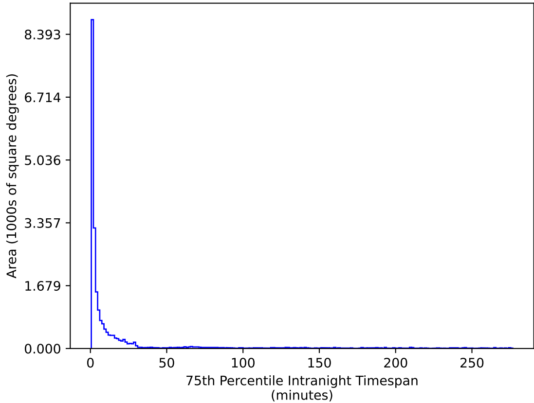
reweight_plane_v3.3_10yrs All sky u band: 75th Percentile Intranight Timespan
