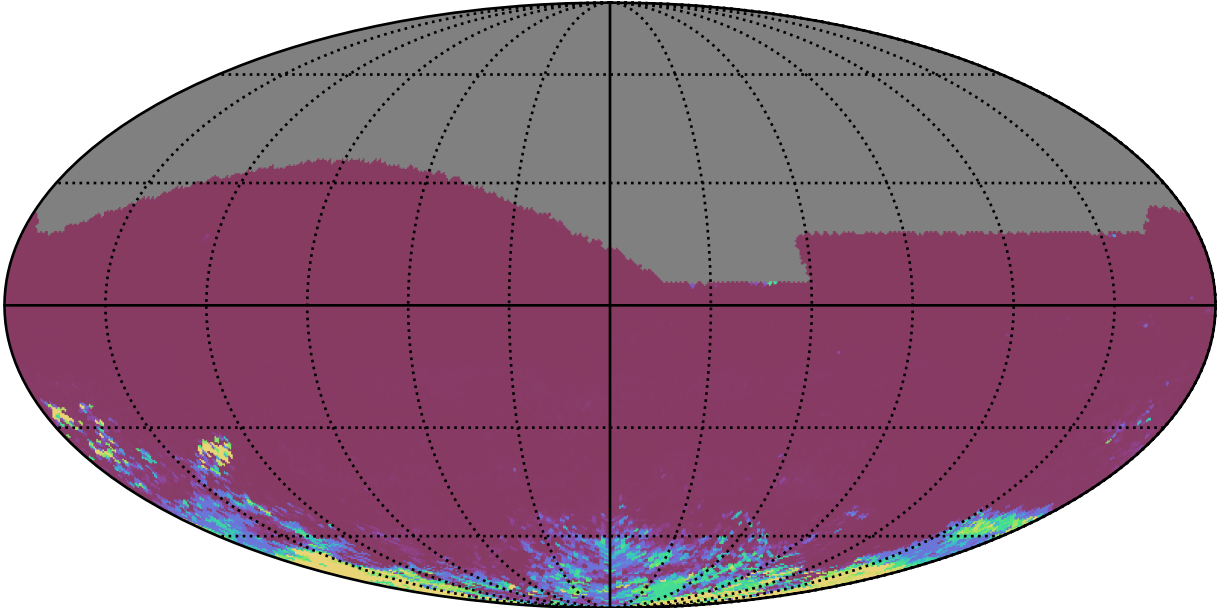
reweight_plane_v3.3_10yrs All sky ri bands: 75th Percentile Intranight Timespan
