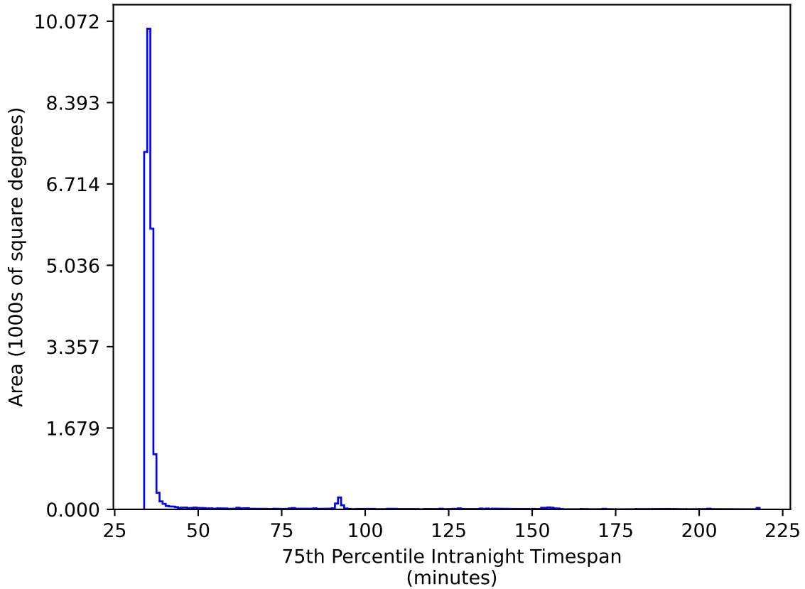
reweight_plane_v3.3_10yrs All sky ri bands: 75th Percentile Intranight Timespan
