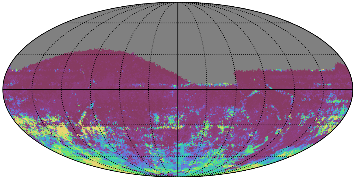
reweight_plane_v3.3_10yrs All sky r band: 75th Percentile Intranight Timespan
