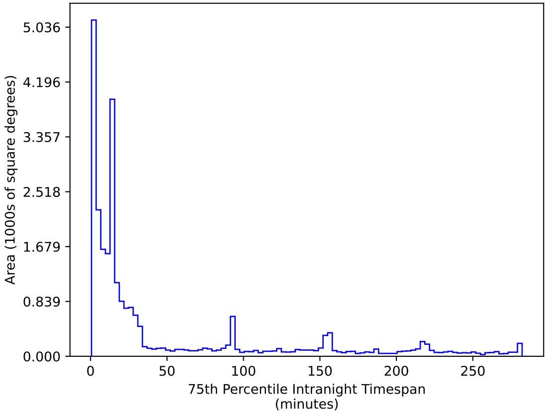
reweight_plane_v3.3_10yrs All sky r band: 75th Percentile Intranight Timespan
