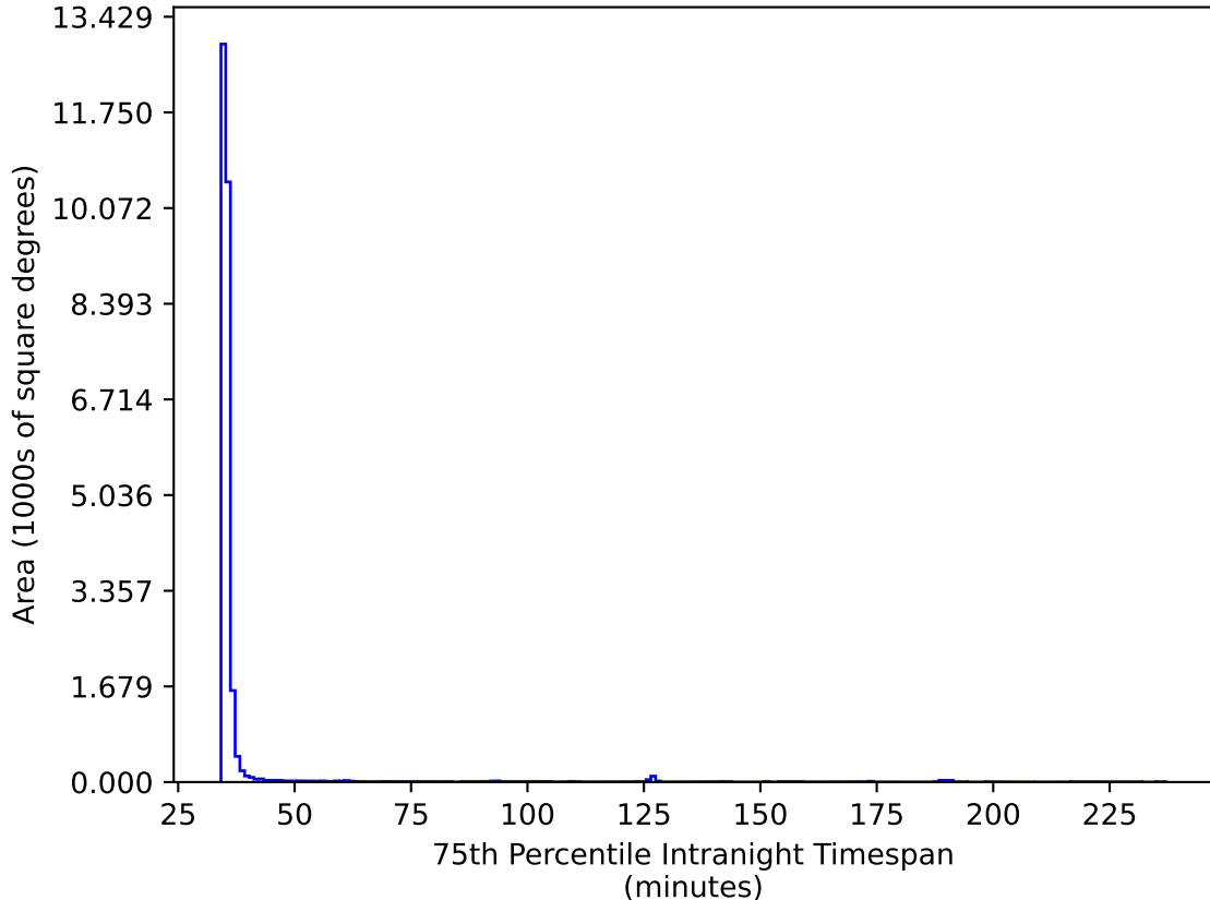
reweight_plane_v3.3_10yrs All sky gr bands: 75th Percentile Intranight Timespan
