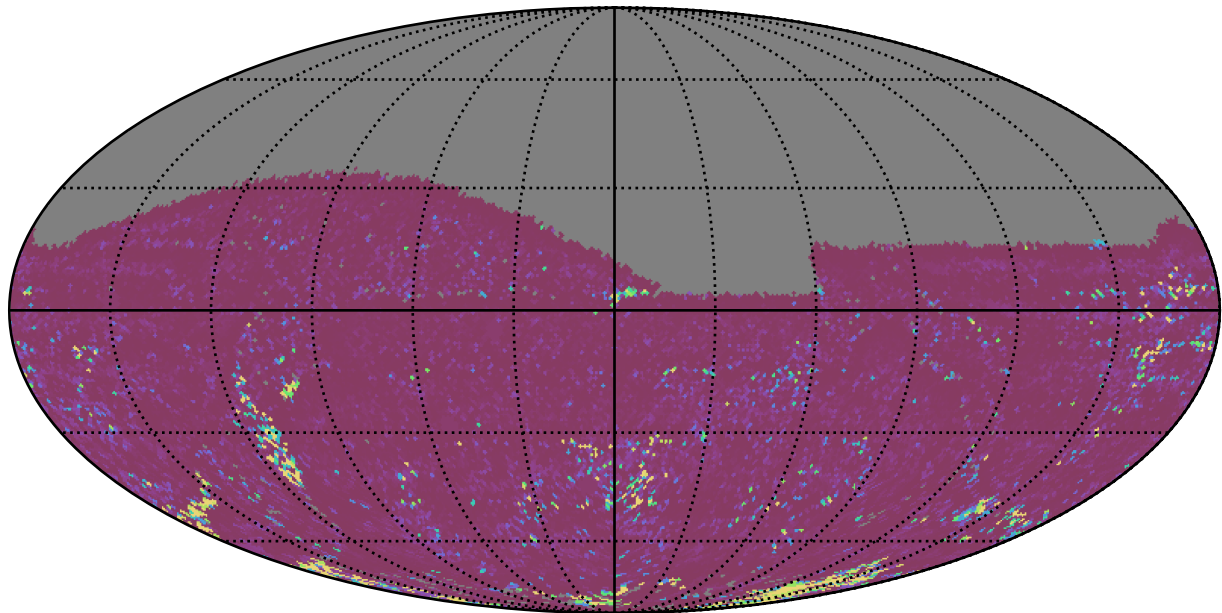
reweight_plane_v3.3_10yrs All sky g band: 75th Percentile Intranight Timespan
