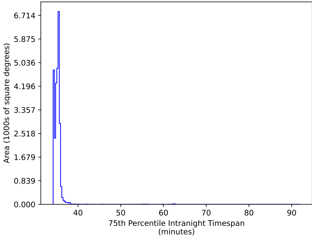
reweight_plane_v3.3_10yrs All sky all bands: 75th Percentile Intranight Timespan
