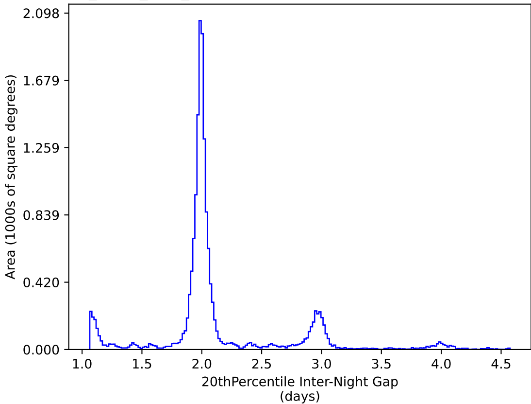
reweight_plane_v3.3_10yrs WFD y band: 20thPercentile Inter-Night Gap
