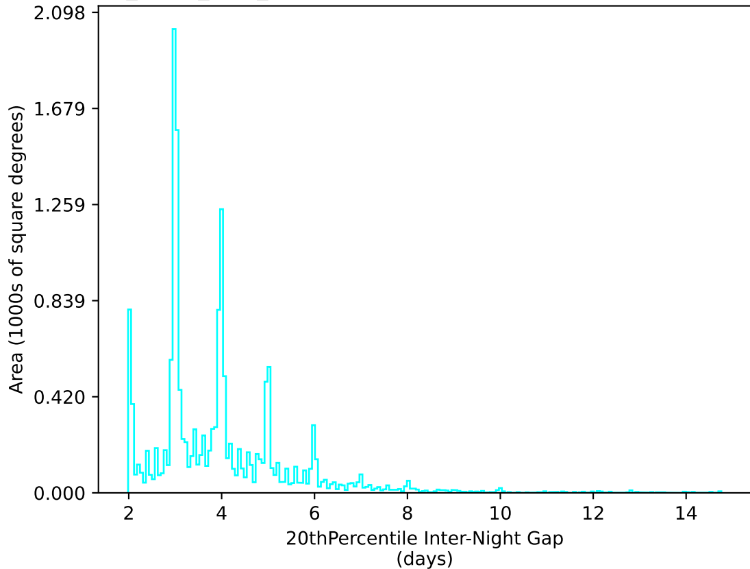
reweight_plane_v3.3_10yrs WFD u band: 20thPercentile Inter-Night Gap
