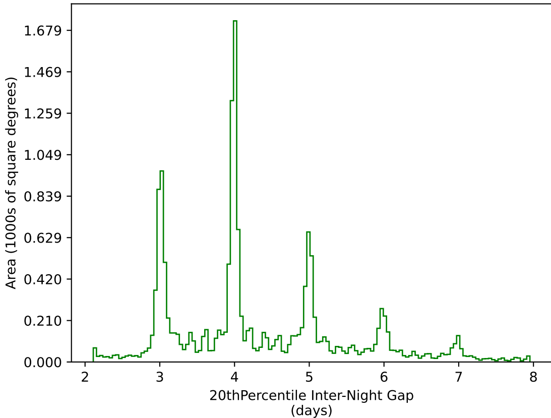
reweight_plane_v3.3_10yrs WFD g band: 20thPercentile Inter-Night Gap
