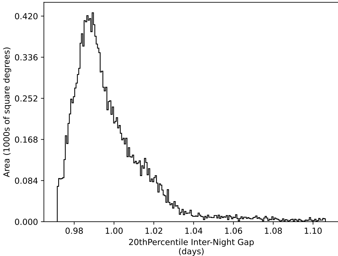
reweight_plane_v3.3_10yrs WFD all bands: 20thPercentile Inter-Night Gap
