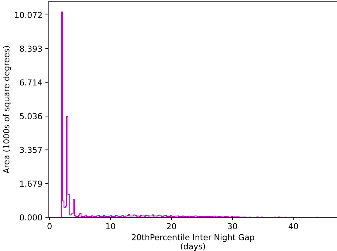
reweight_plane_v3.3_10yrs All sky z band: 20thPercentile Inter-Night Gap
