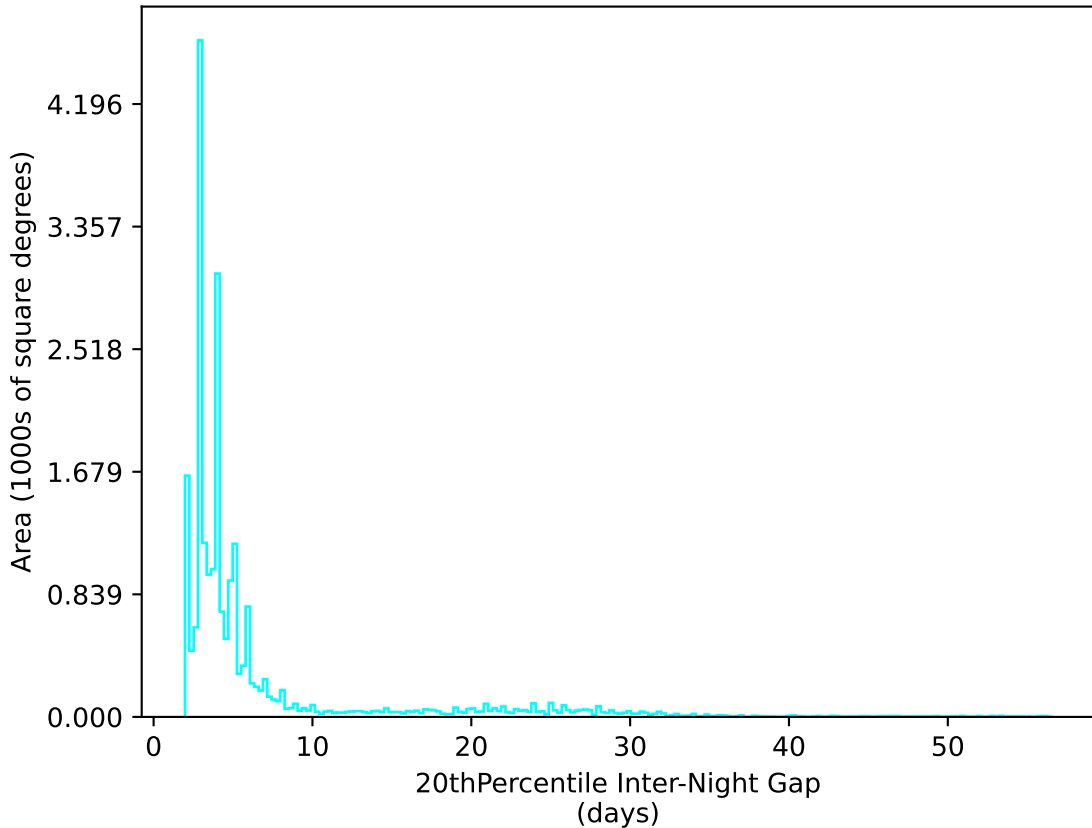
reweight_plane_v3.3_10yrs All sky u band: 20thPercentile Inter-Night Gap
