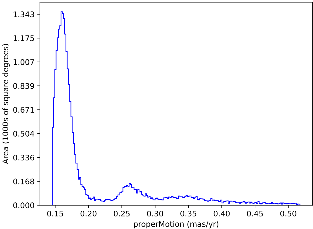
reweight_plane_v3.3_10yrs : properMotion
