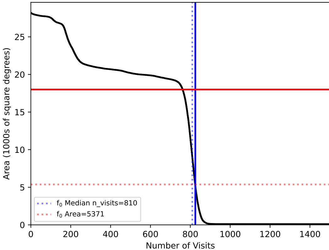
reweight_plane_v3.3_10yrs : f0
