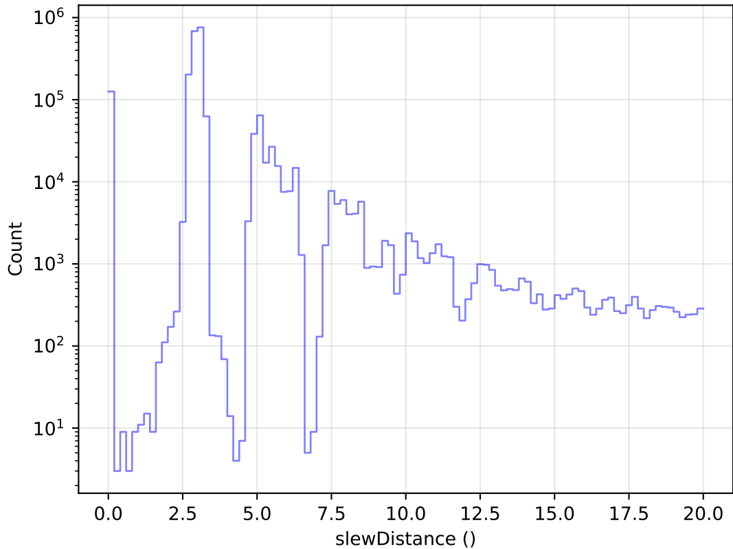
reweight_plane_v3.3_10yrs All visits: Zoom Slew Distance Histogram
