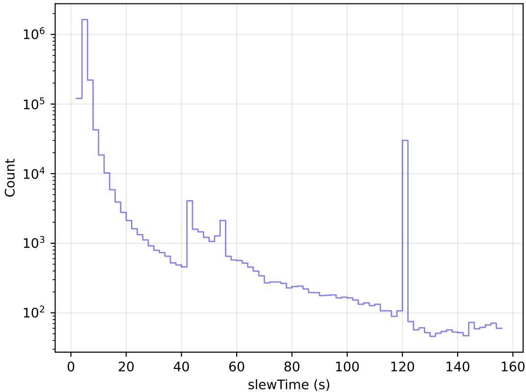
reweight_plane_v3.3_10yrs All visits: Slew Time Histogram
