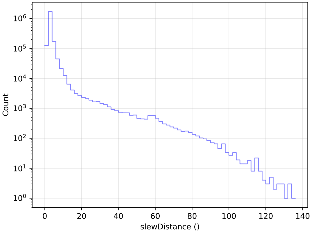
reweight_plane_v3.3_10yrs All visits: Slew Distance Histogram
