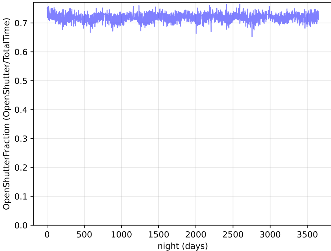
reweight_plane_v3.3_10yrs : OpenShutterFraction
