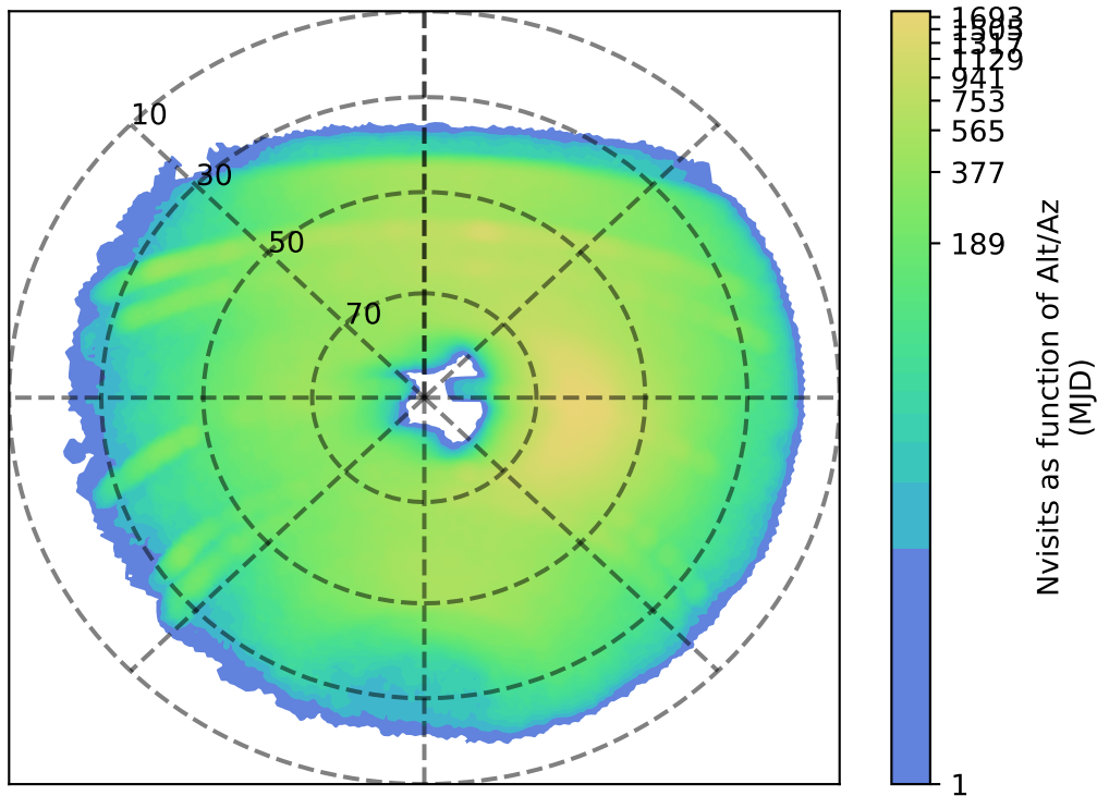
reweight_plane_v3.3_10yrs y: Nvisits as function of Alt/Az
