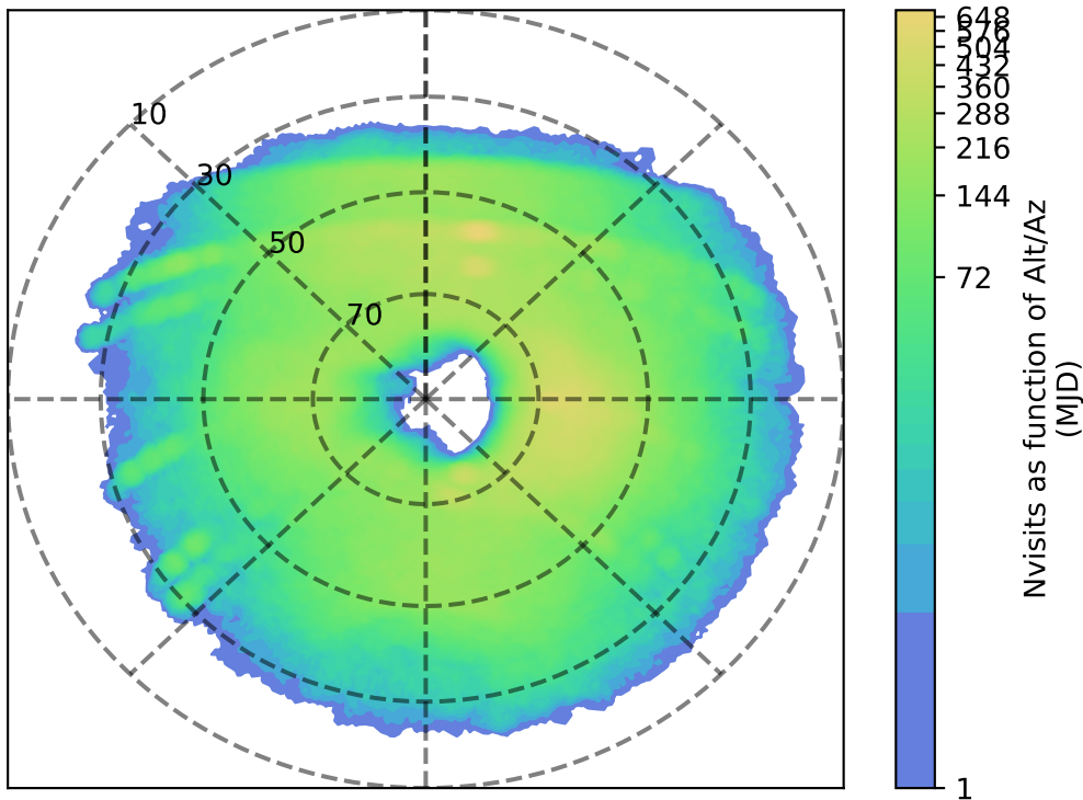
reweight_plane_v3.3_10yrs u: Nvisits as function of Alt/Az
