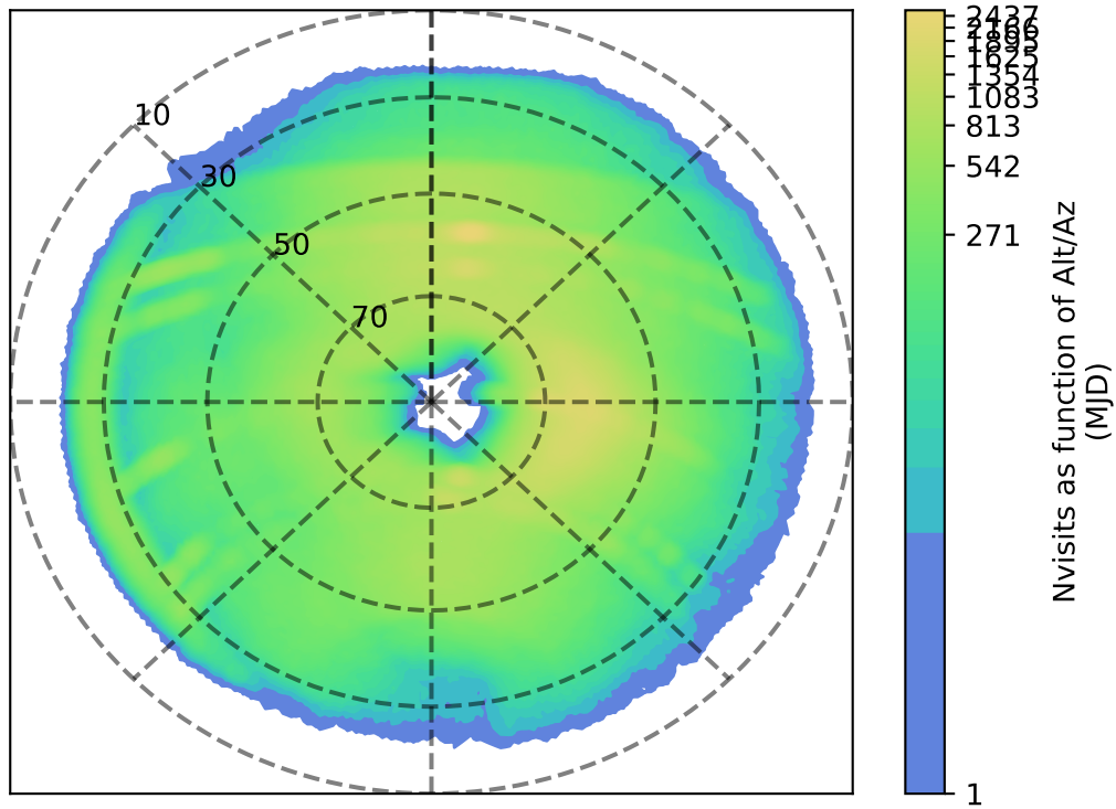
reweight_plane_v3.3_10yrs r: Nvisits as function of Alt/Az
