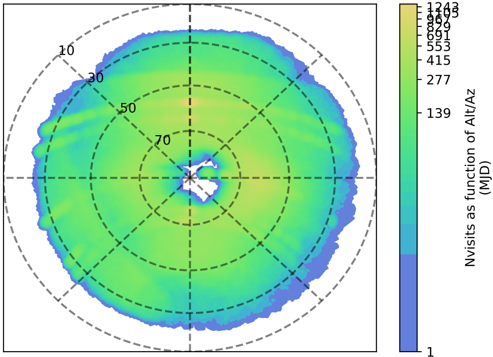
reweight_plane_v3.3_10yrs g: Nvisits as function of Alt/Az
