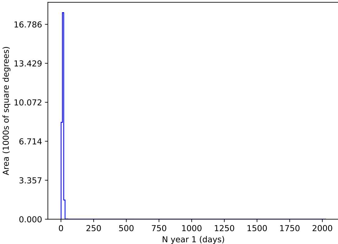
reweight_plane_v3.3_10yrs z and night < 365: N year 1
