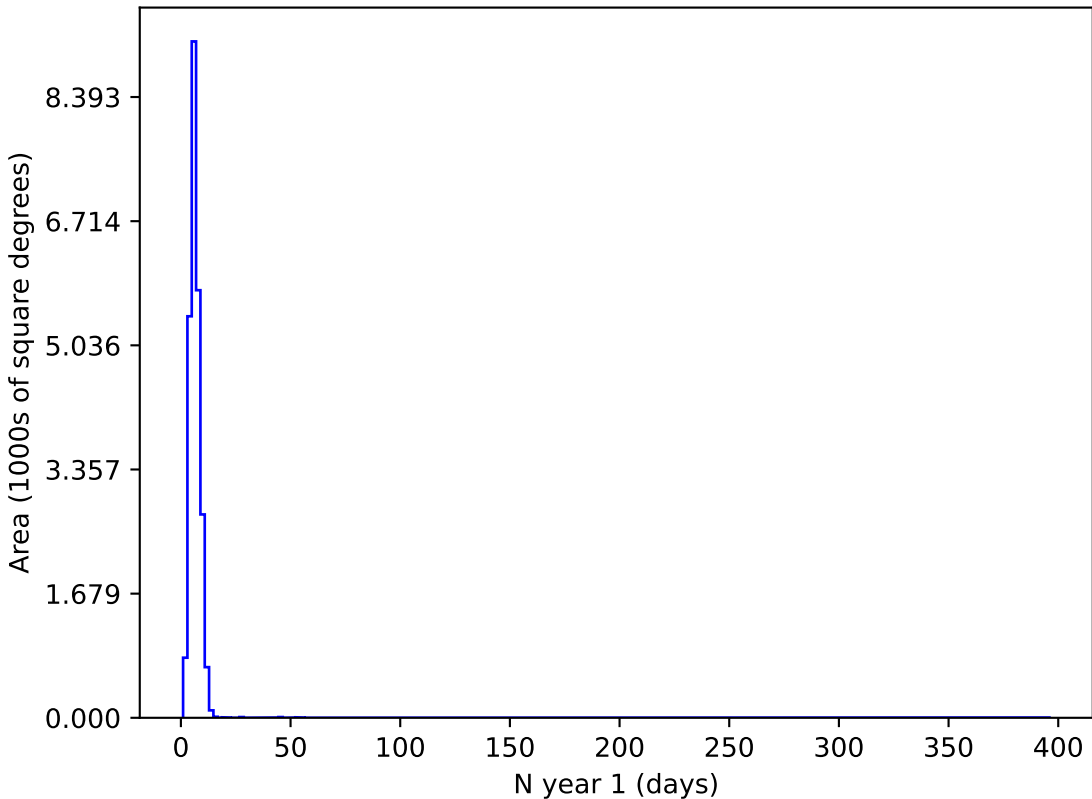
reweight_plane_v3.3_10yrs u and night < 365: N year 1
